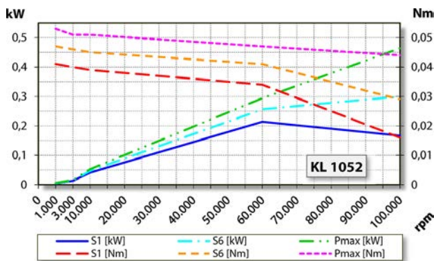
Performance Diagram Compressed air cooled
