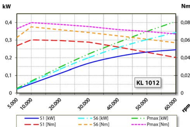
Performance Diagram Uncooled
