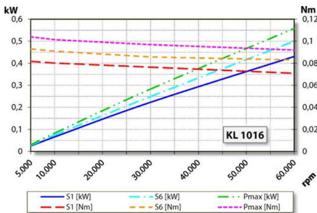
Performance Diagram Spindle holder cooled
